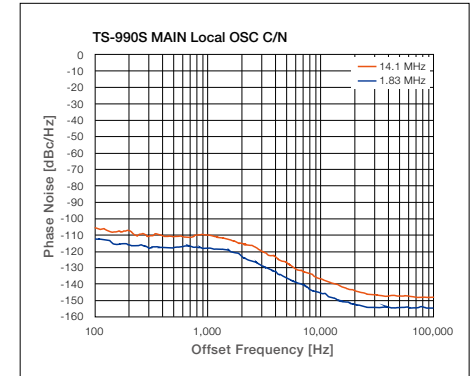
Main receiver 1st Local Oscillator C/N Main receiver characteristic example (20m/160m)
