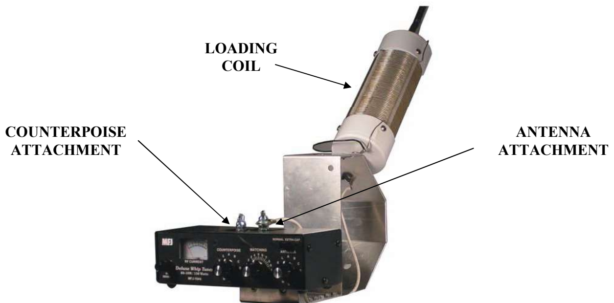
Figure 1: MFJ-1625 Window/Balcony Mount Antenna
