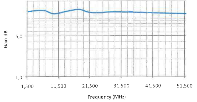
MLA100 Typical Gain vs Frequency
