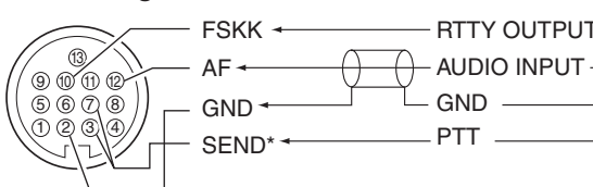
Rear panel view
